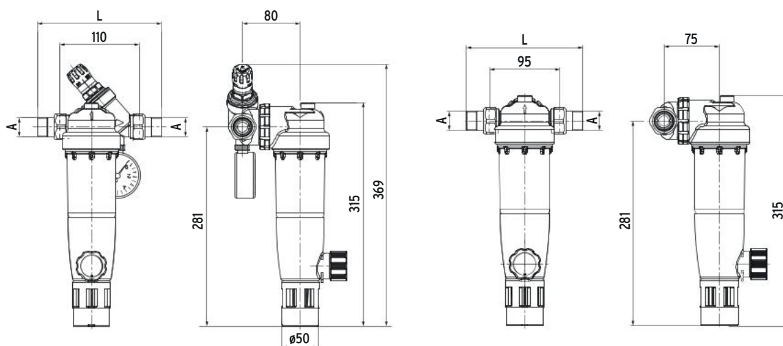
Maße [mm]
