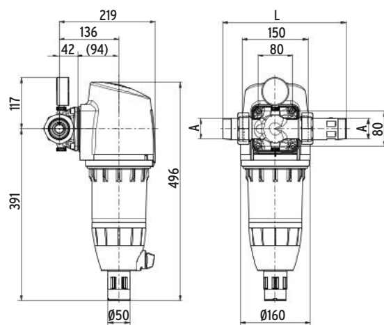
Maße [mm]
