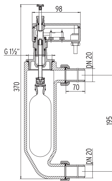
Maße [mm]
