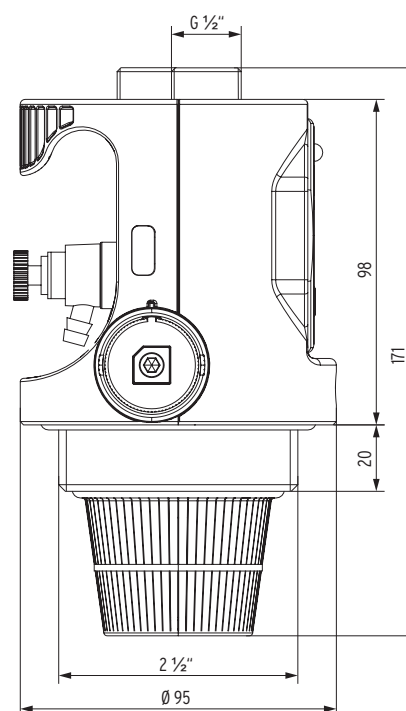
Maße [mm]
