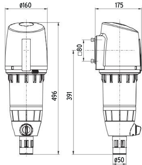
Maße [mm]
