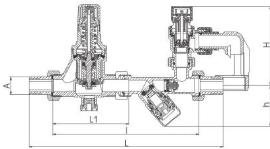
SYRobloc 25, DN 15
