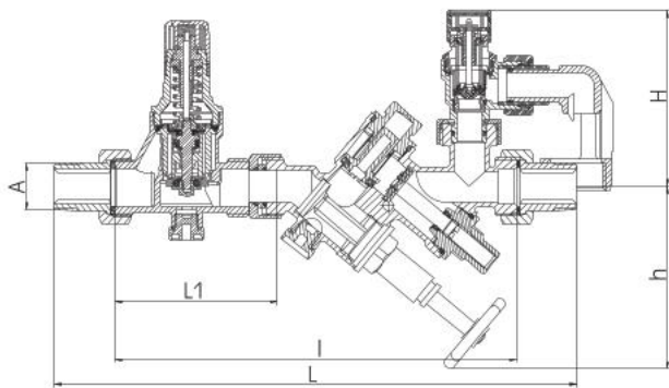
SYRobloc 25, DN 20
