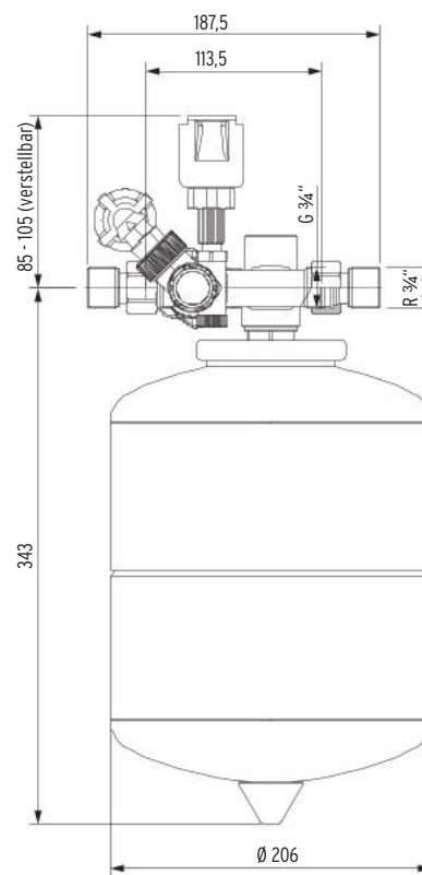
Maße [mm]
