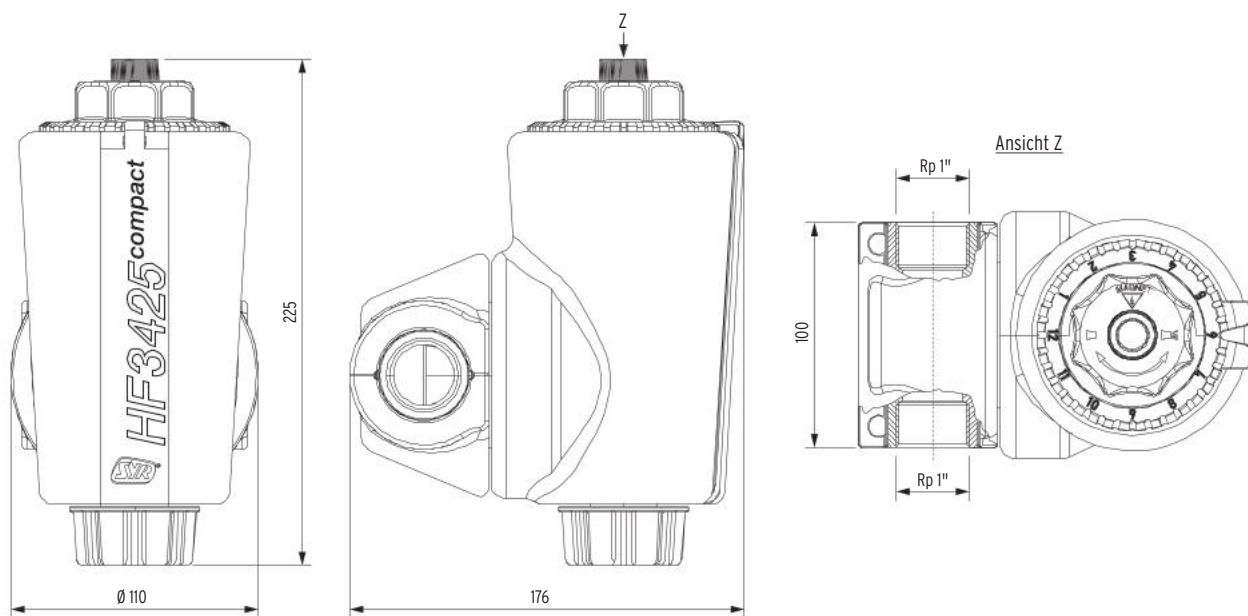
Maße [mm]
